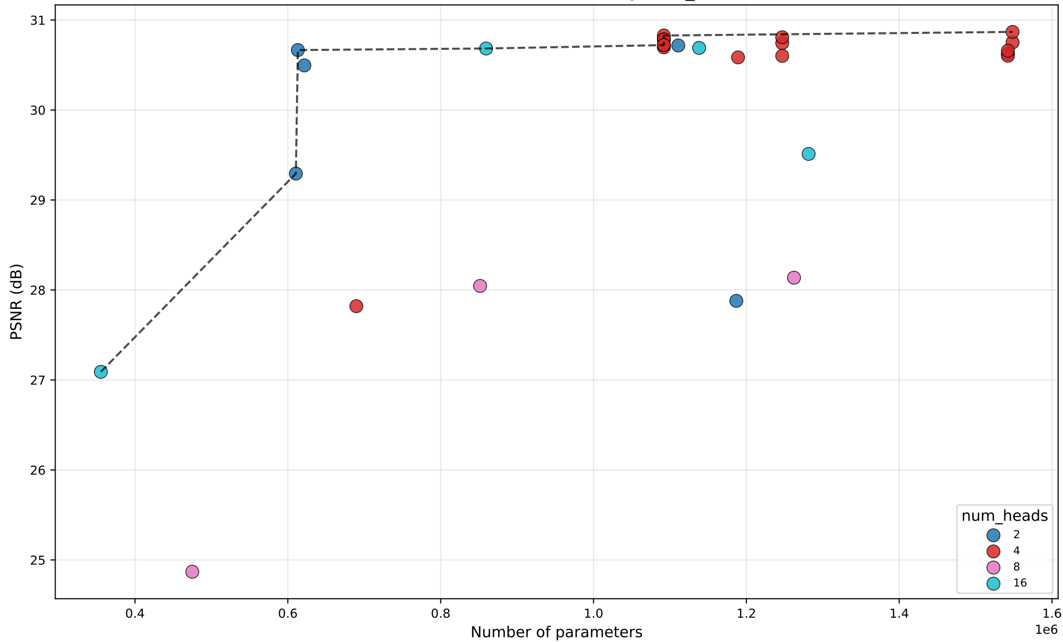
PSNR vs #Params — HAT — by num_heads
